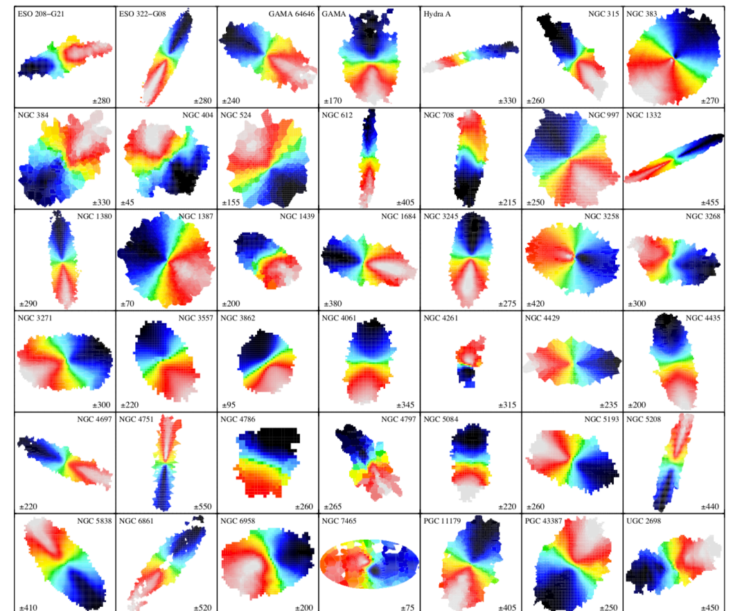
ALMA CO imaging of early-type galaxies
